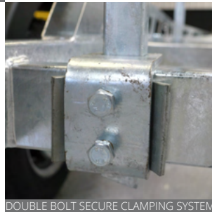
DOUBLE BOLT SECURE CLAMPING SYSTEM
